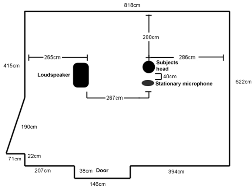
Figure 1: The silent low reverberation room where the study was conducted
