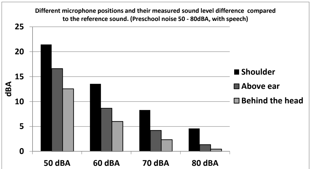
Figure 5: Background noise measurements using preschool noise with speech contribution from the microphone carrier compared to reference measurement
