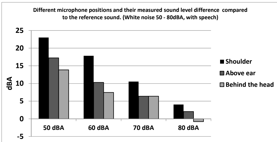
Figure 3: Background noise measurements using white noise with speech contribution from the microphone carrier compared to reference measurement
