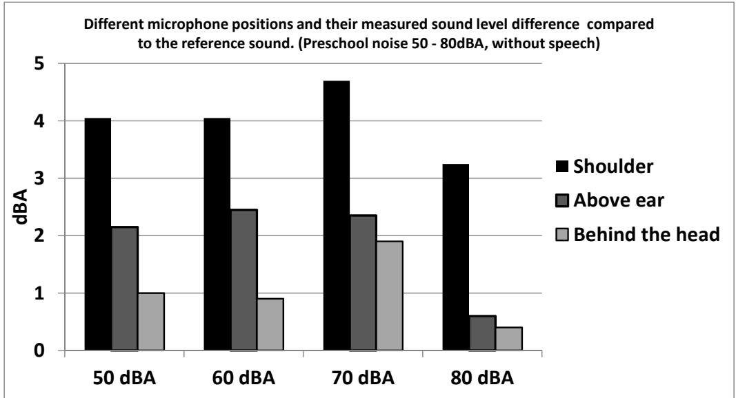
Figure 4: Background noise measurements using preschool noise compared to reference measurement
