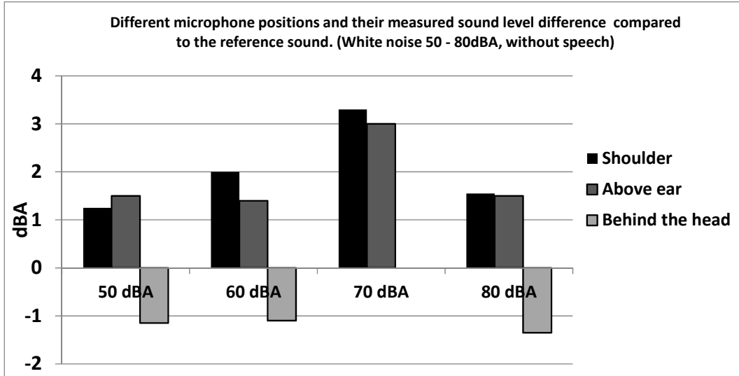
Figure 2: Background noise measurements using white noise compared to reference measurement
